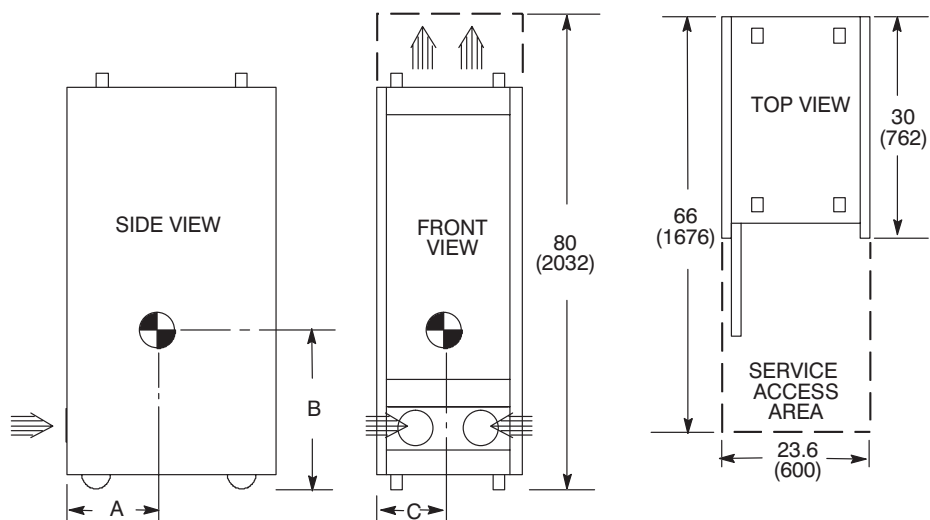
SERVICE AND VENTILATION CLEARANCE ILLUSTRATION 2–2
